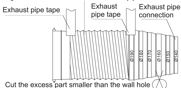
Figure 4 Ø185 aluminum foil exhaust pipe
