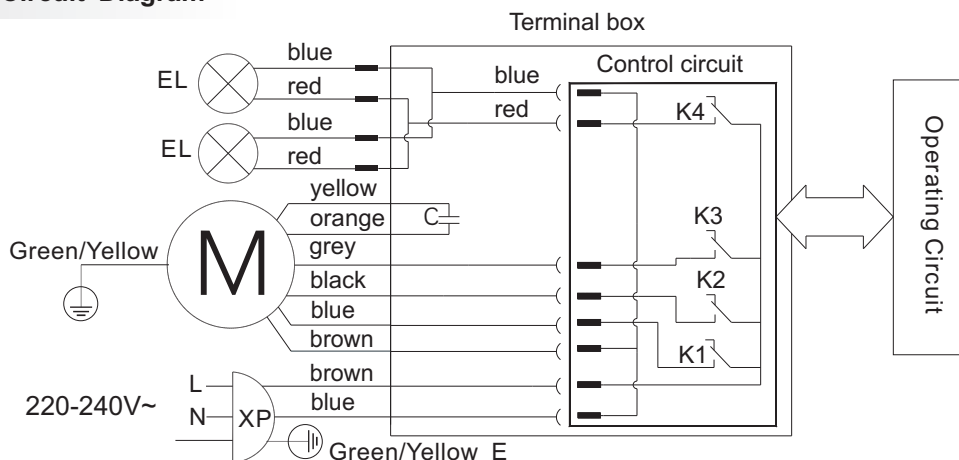
A815 Circuit Diagram
