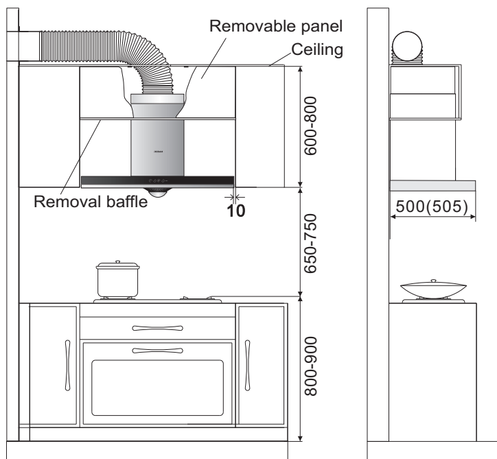
(Figure 1-2 Installation method of hood with removable baffle) (Figures in brackets are specific to the A815 hood)
