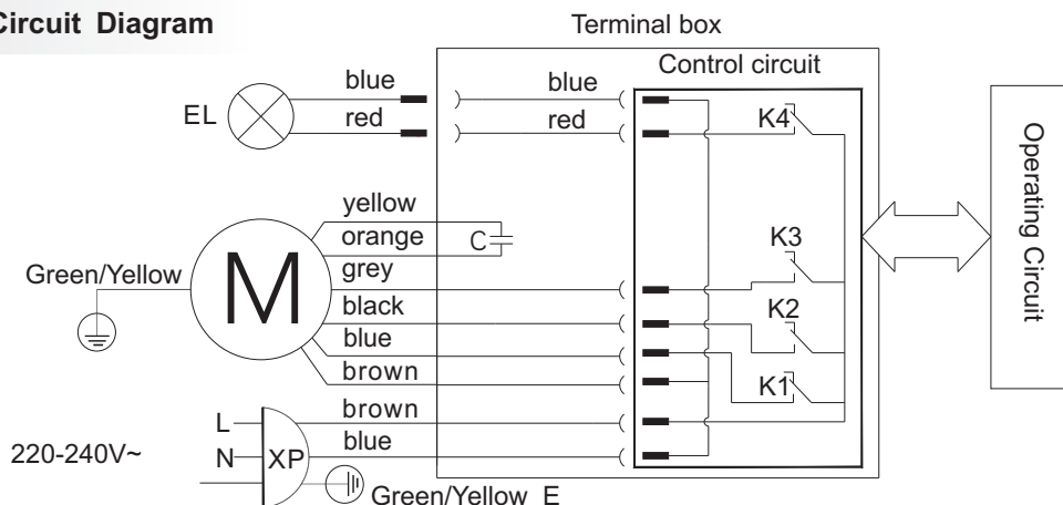
A815 Circuit Diagram
